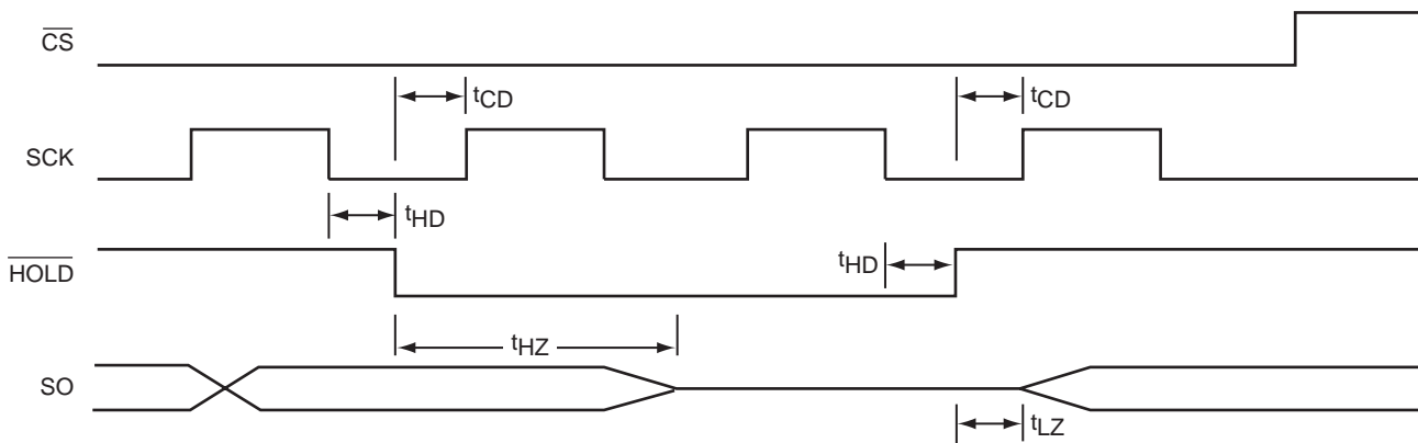
Figure 9. \overline{HOLD} Timing
