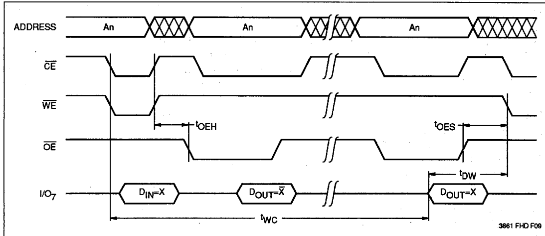
DATA Polling Timing Diagram (9)
