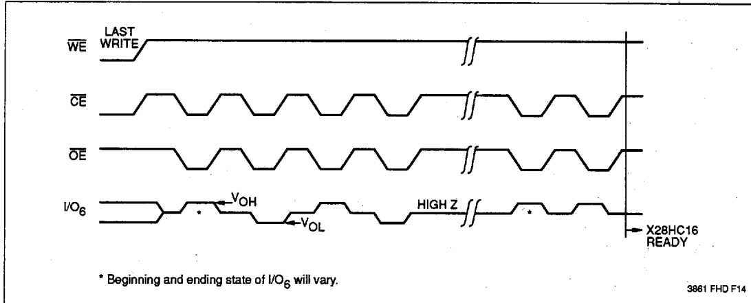
THE TOGGLE BIT I/O, Figure 4. Toggle Bit Bus Sequence
