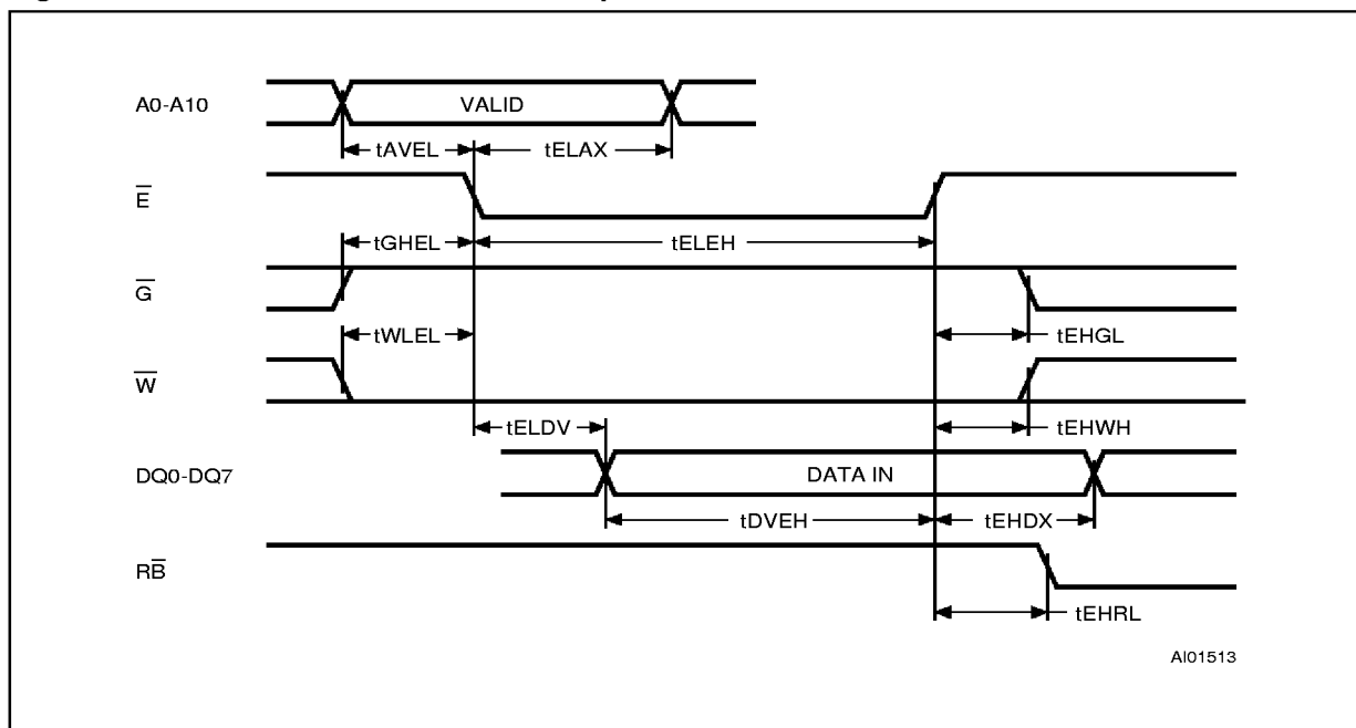
Figure 11. Write Mode AC Waveforms - Chip Enable Controlled
