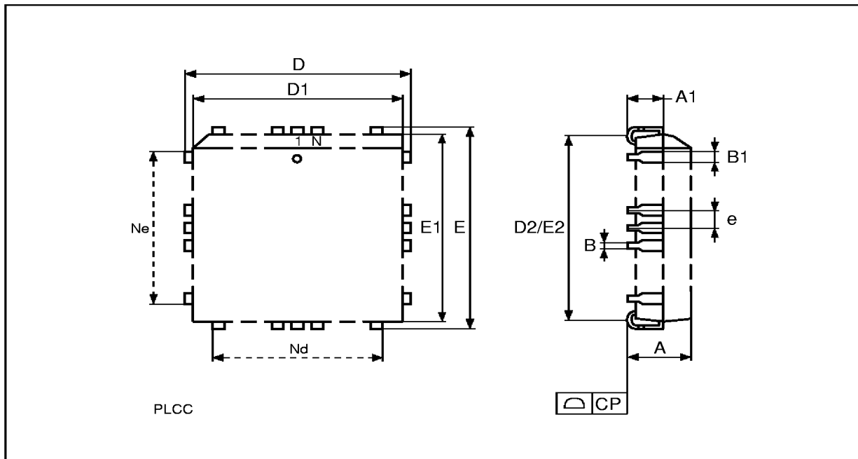
PLCC32
