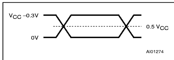
Figure 7. AC Testing Input Output Waveforms
