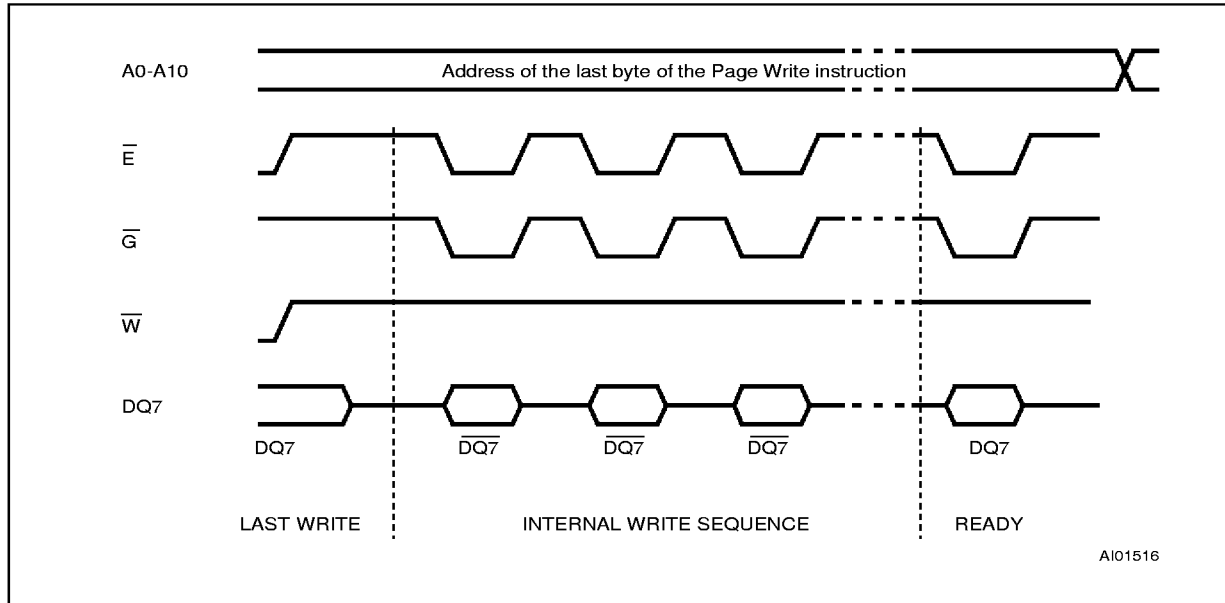
Figure 14. Data Polling Waveform Sequence
