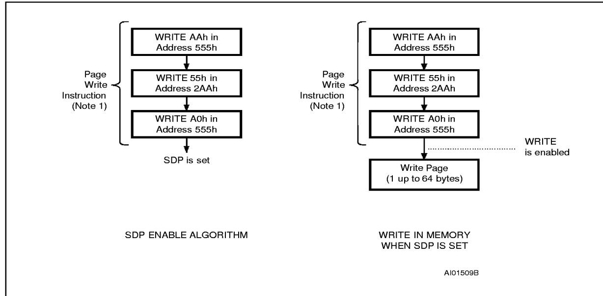
Figure 5. Software Data Protection Enable Algorithm and Memory Write
