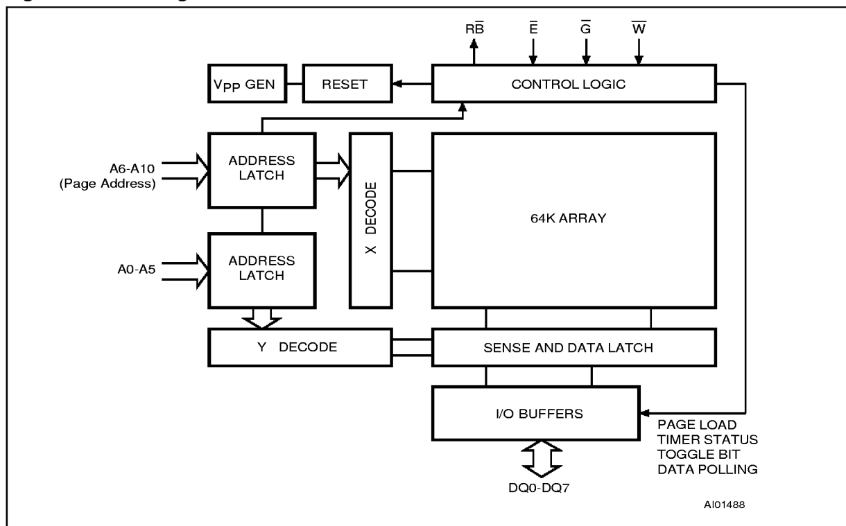
Figure 3. Block Diagram
