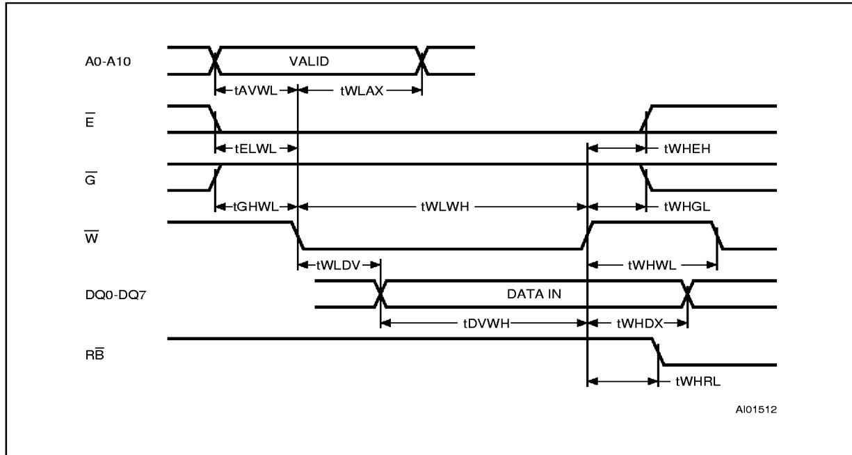
Figure 10. Write Mode AC Waveforms - Write Enable Controlled
