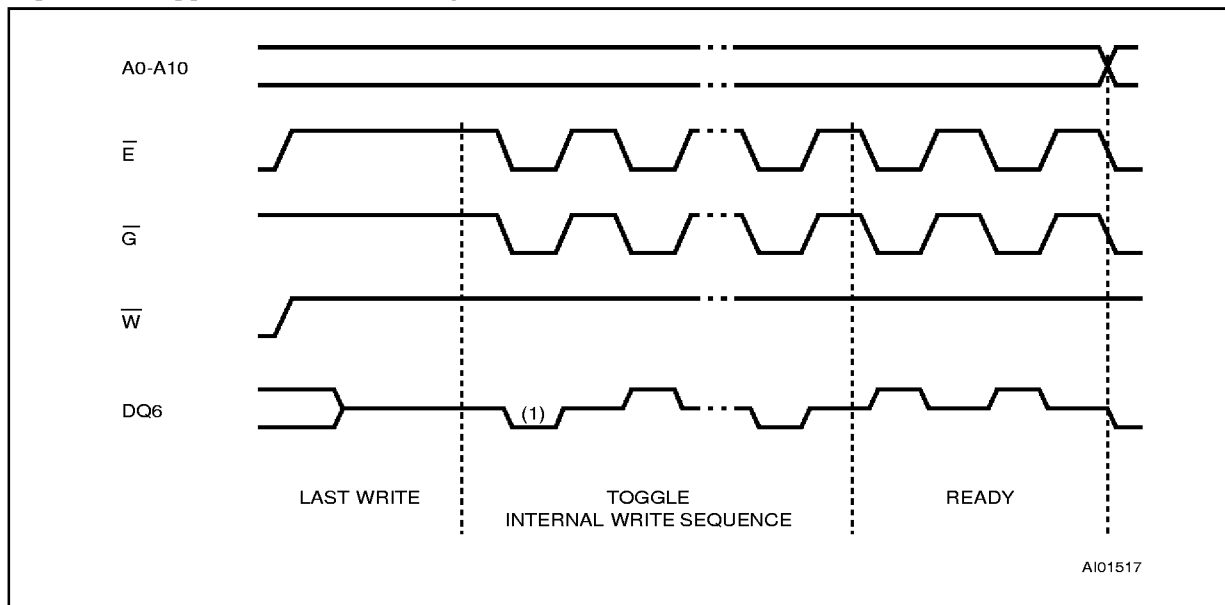
Figure 15. Toggle Bit Waveform Sequence
