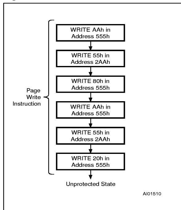
Figure 6. Software Data Protection Disable Algorithm
