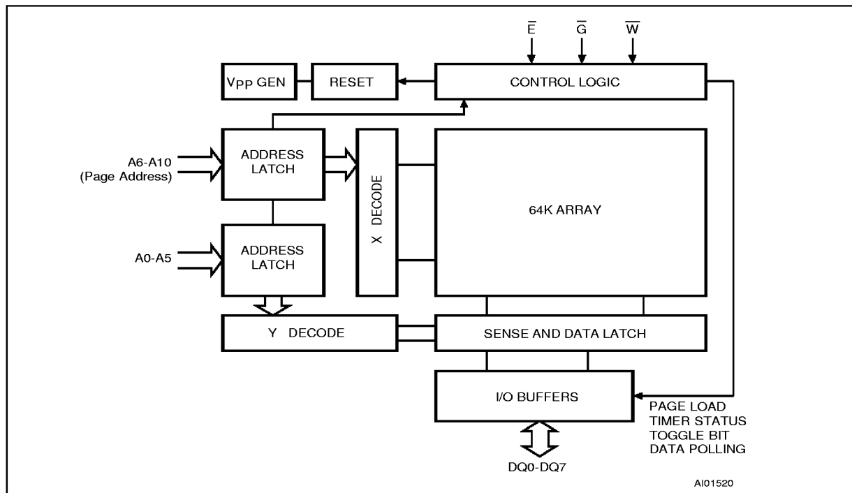
Figure 3. Block Diagram
