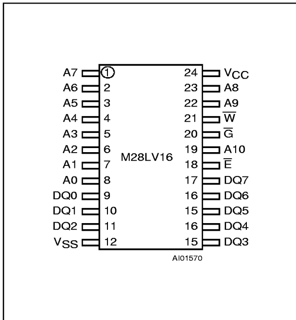
Figure 2C. SO Pin Connections
