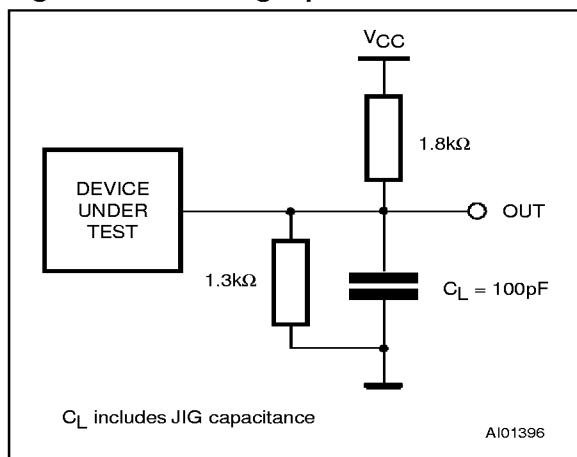
Figure 8. AC Testing Equivalent Load Circuit
