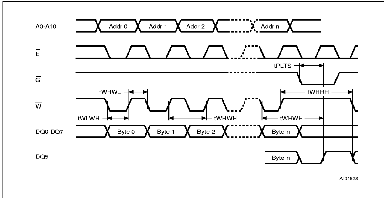
Figure 12. Page Write Mode AC Waveforms - Write Enable Controlled
