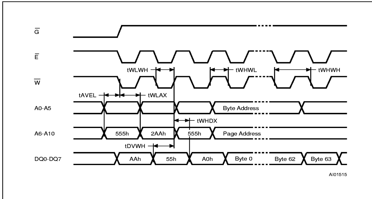
Figure 13. Software Protected Write Cycle Waveforms
