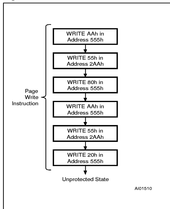
Figure 6. Software Data Protection Disable Algorithm
