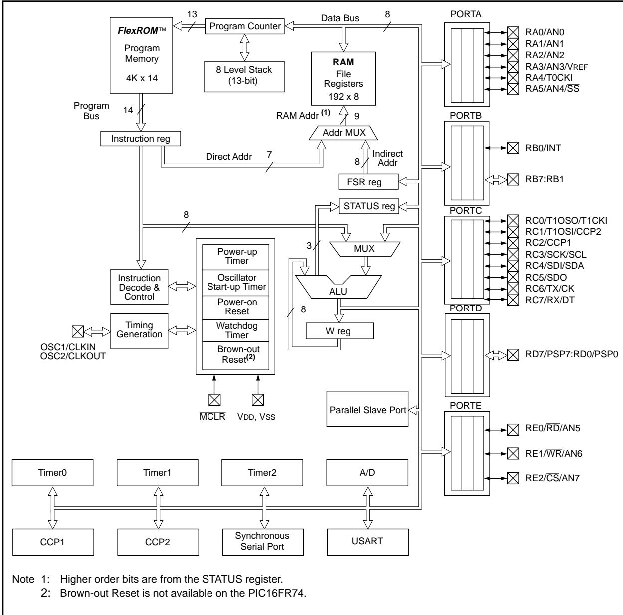
FIGURE 5-2: PIC16FR74/74A BLOCK DIAGRAM
