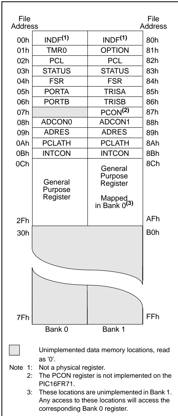
FIGURE 2-5: PIC16FR710/71 REGISTER FILE MAP
