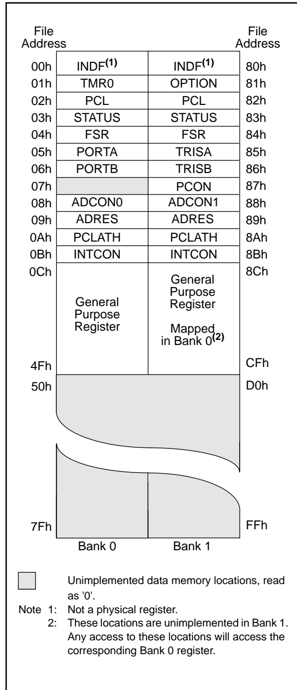
FIGURE 2-6: PIC16FR711 REGISTER FILE MAP
