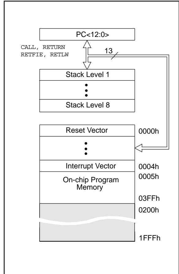
FIGURE 2-4: PIC16FR711/711 PROGRAM MEMORY MAP AND STACK
