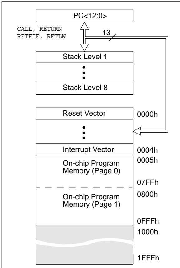
FIGURE 4-3: PIC16FR73/73A PROGRAM MEMORY MAP AND STACK
