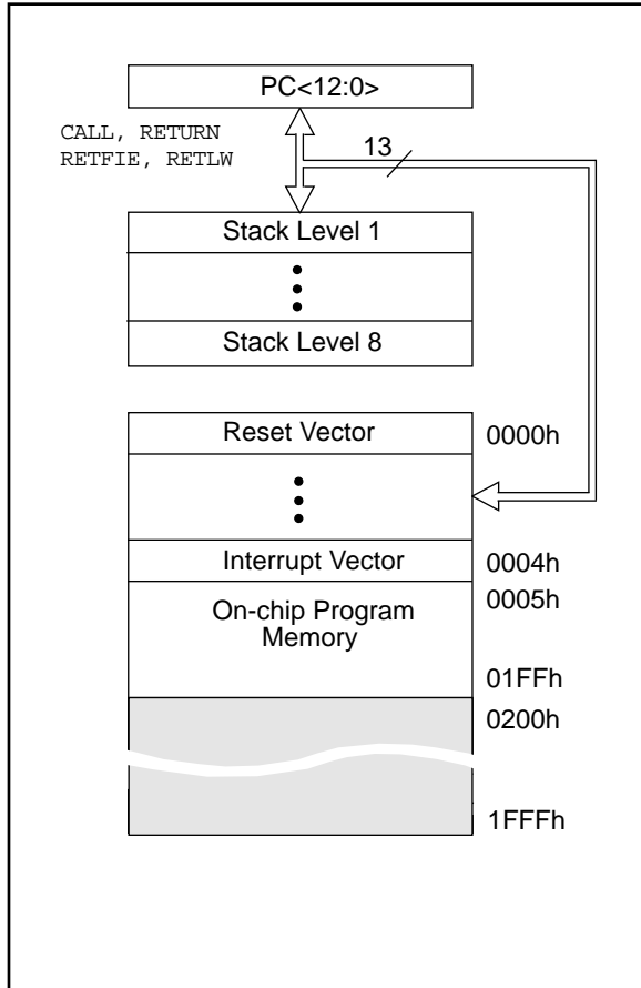
FIGURE 2-3: PIC16FR710 PROGRAM MEMORY MAP AND STACK
