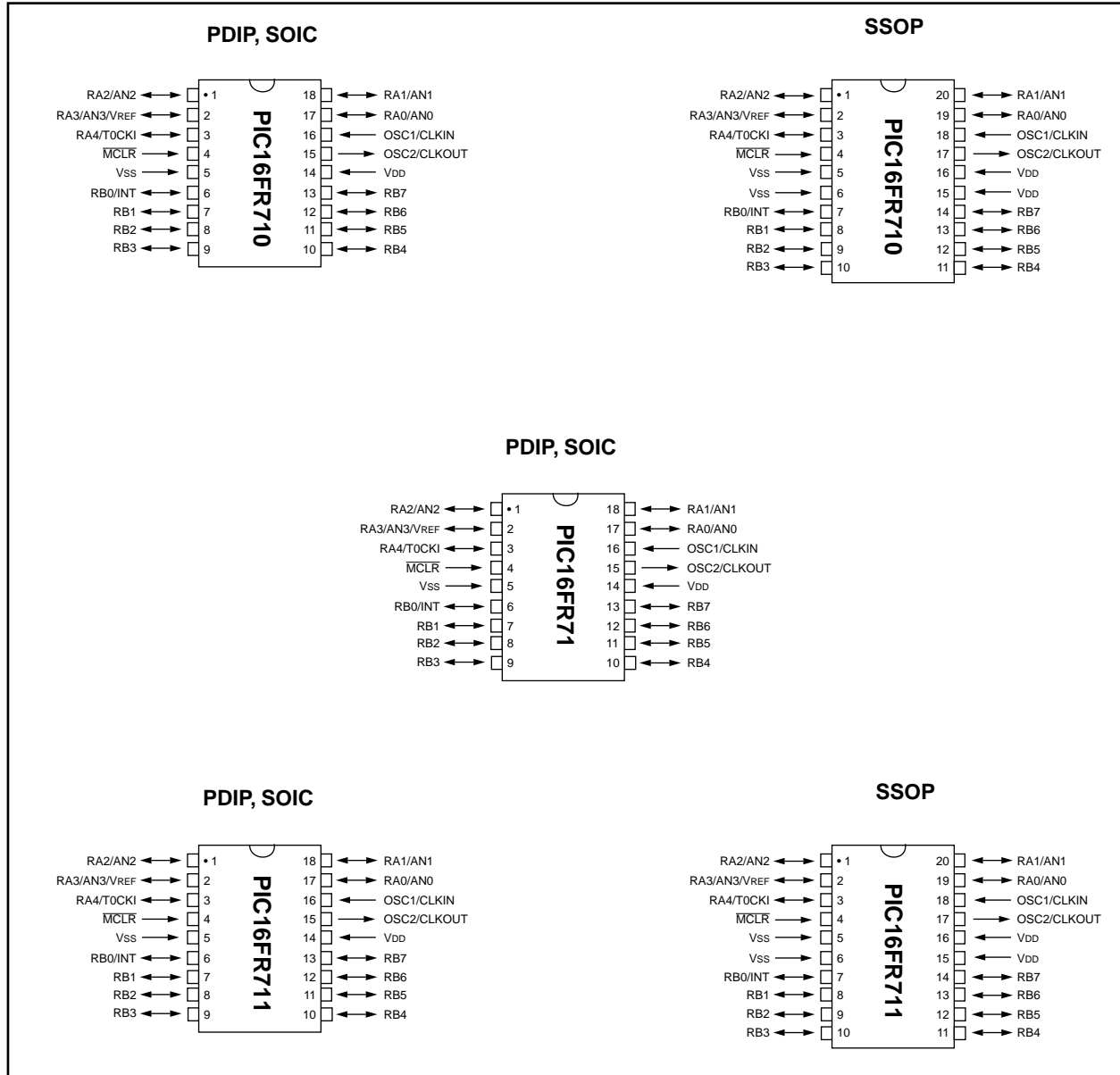
FIGURE 2-1: PIN DIAGRAMS
