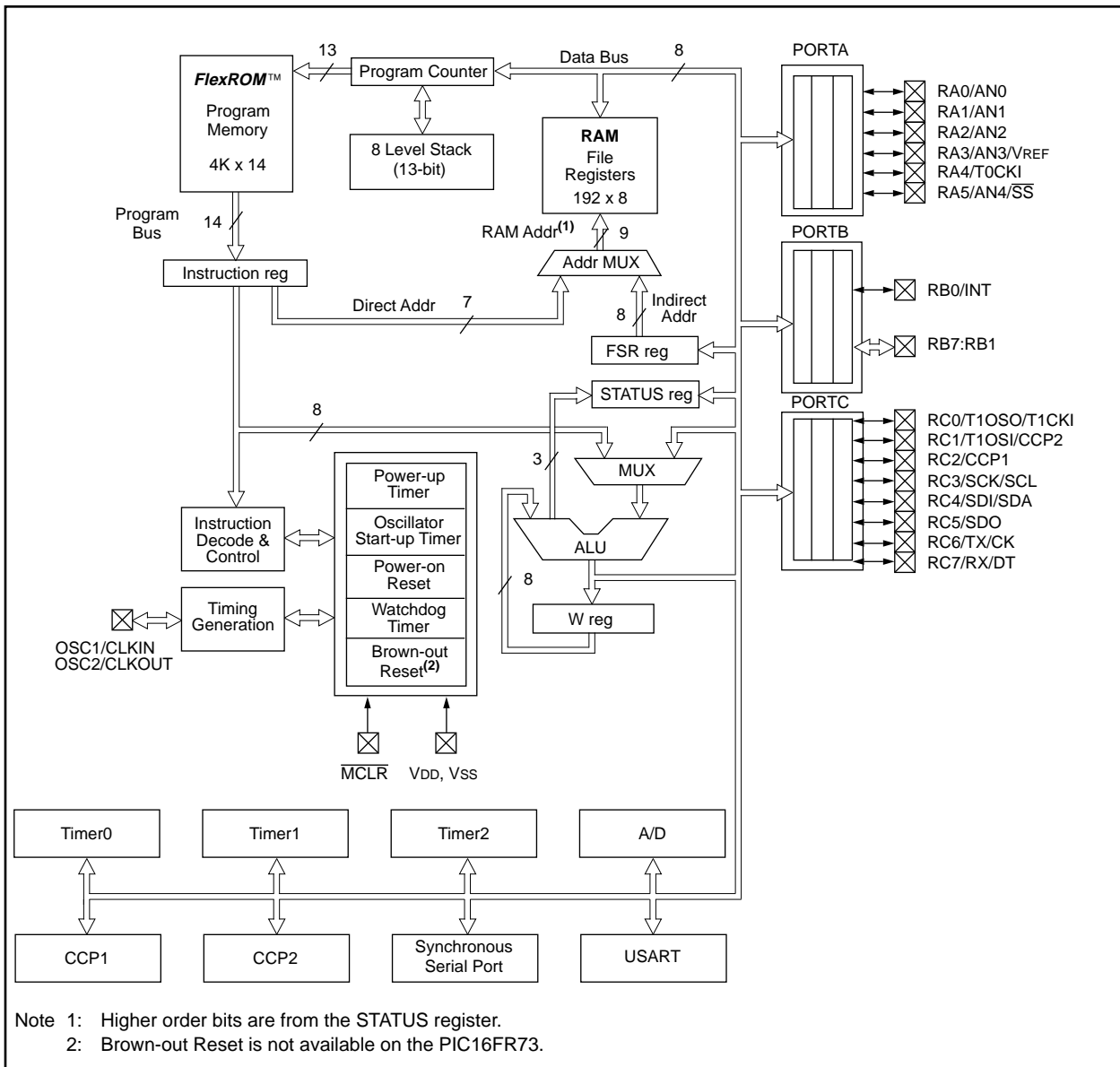
FIGURE 4-2: PIC16FR73/73A BLOCK DIAGRAM
