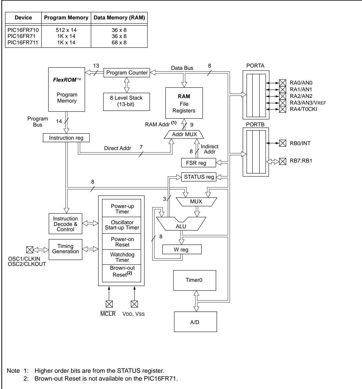
FIGURE 2-2: PIC16FR710/71/711 BLOCK DIAGRAM
