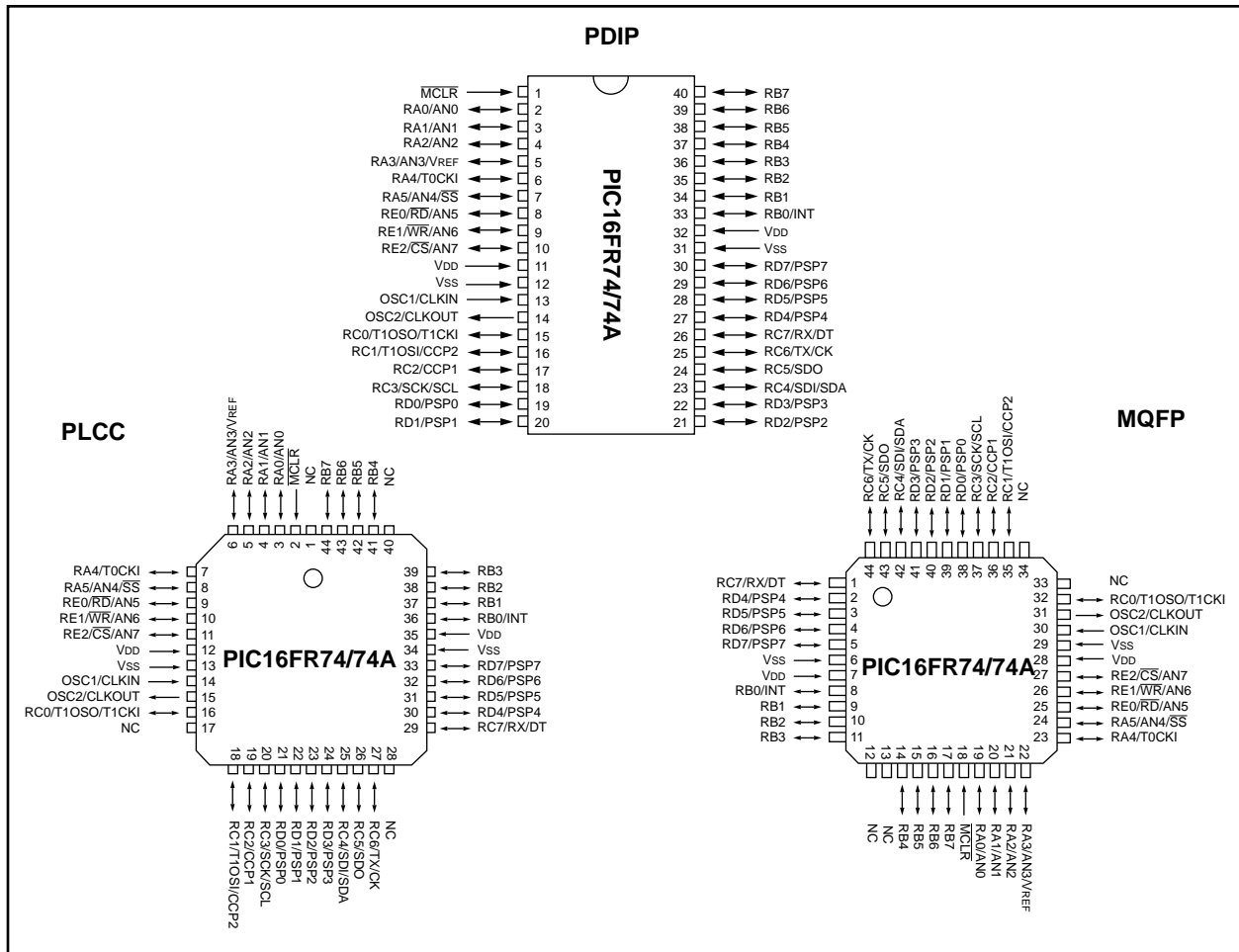
FIGURE 5-1: PIC16FR74/74A PIN DIAGRAMS
