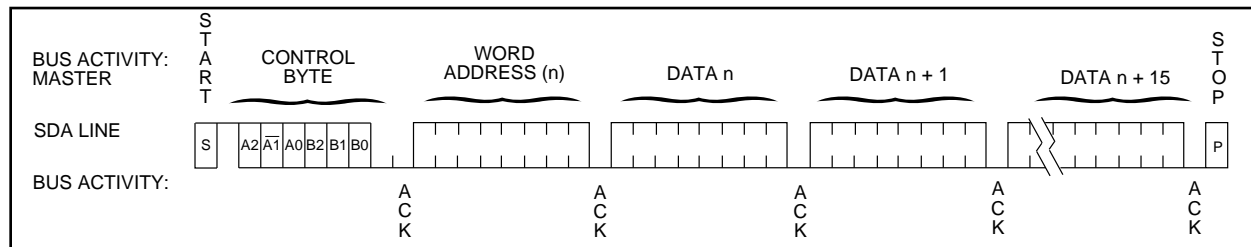
FIGURE 4-2: PAGE WRITE
